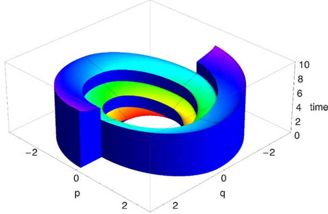
Figure 6. The shortest times necessary to reach the target energy E_T = 1/2 (bottom ellipse) of a classical harmonic oscillator starting from initial states (q_i, p_i) . The optimal paths use the two frequencies \omega_{\max} = \sqrt{2} and \omega_{\min} = 1 , and the target energy is computed with \omega_T = \omega_{\min} . The vertical cliffs are the resonant trajectories.
